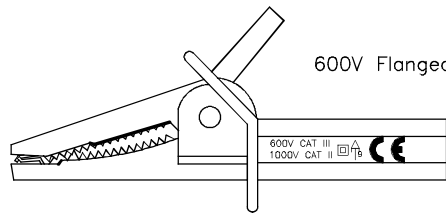
600V Flanged Croc. Clip: 126009R
